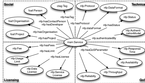
Fig. 1. A partial view of the SmartLink NfP Schema.
