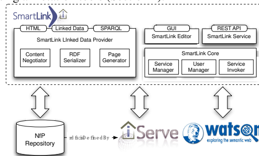
Fig. 2. SmartLink – overall architecture.
